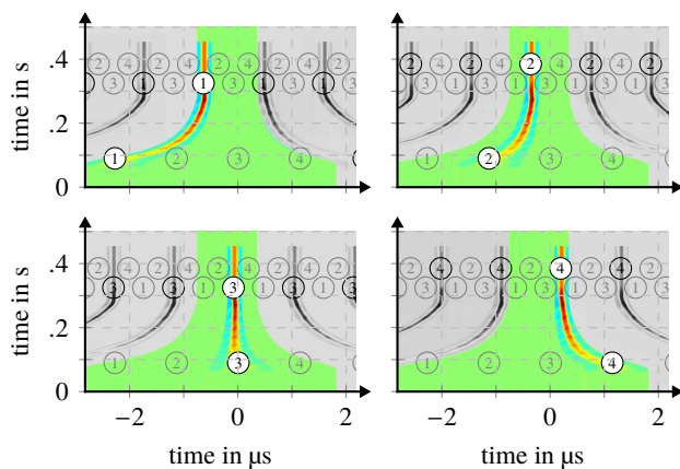
Figure 2: Tracking of single bunches during acceleration, full machine cycle, 11.4 - 1000 MeV/u (maximum rigidity). Only one revolution colored.
