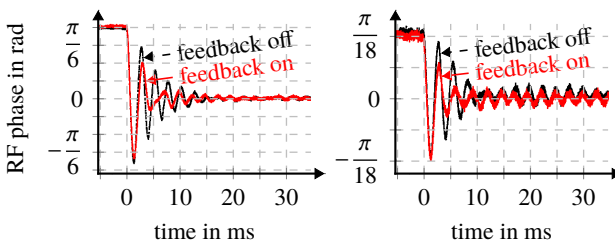
Figure 5: Comparison of open and closed loop operation.
