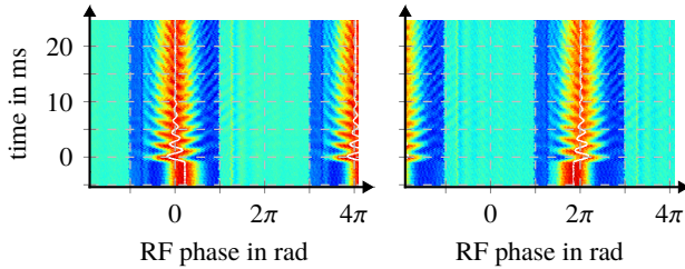
Figure 3: Waterfall plot of single bunches at h=2 with bunch-by-bunch phase detection \Delta\varphi (white lines) using one DSP system per bunch for an out-of-phase excitation.
