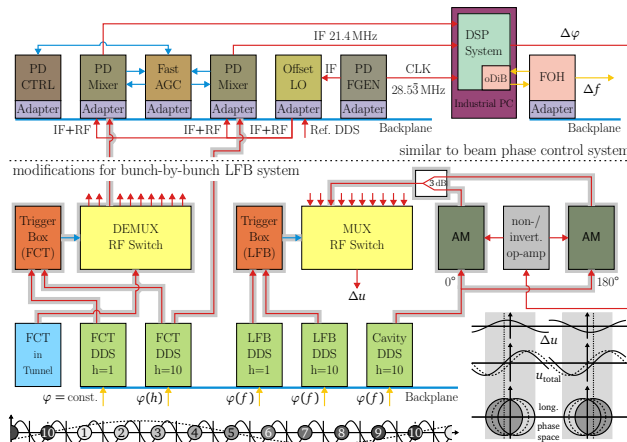
Figure 1: Sketch of LLRF of beam phase control system (top) with modifications for the LFB system (center) and principles of operation (bottom). 1
