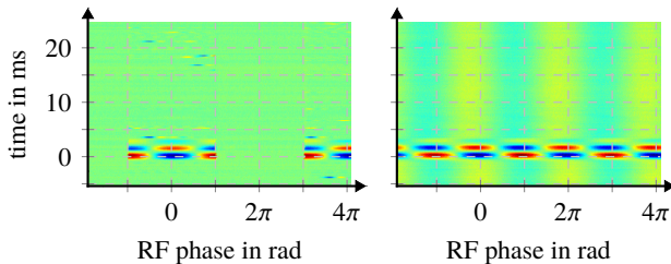
Figure 4: Multiplexed LLRF correction signal \Delta u (left) and resulting gap voltage in a ferrite cavity (right).
